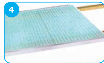
4 Apply a border of aluminum 16mm U-Channel, in conjunction with a bead of Polycarbonate compatible sealant to finish the edges.
