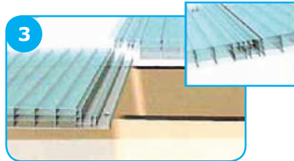
3 Match the next sheet edges carefully and press into place with a "click."
